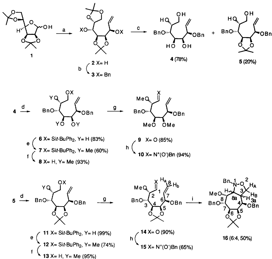
Scheme 2. Reagents: (a) BrMgCH=CH 2 , THF (2:epi-(C-1)-2/ 4:1;75%; separate isomers); (b) BnBr, NaH, THF (85%); (c) AcOH:H 2 O (4:1), 0.2 M, 55 °C; (d) ClSi t -BuPh 2 , py; (e) MeI, NaH, THF; (f) Bu 4 NF, THF; (g) PCC, NaOAc, molecular sieves; (h) NaHCO 3 , EtOAc, HONHBn. HCl; (i) Chlorobenzene, 130 °C.
